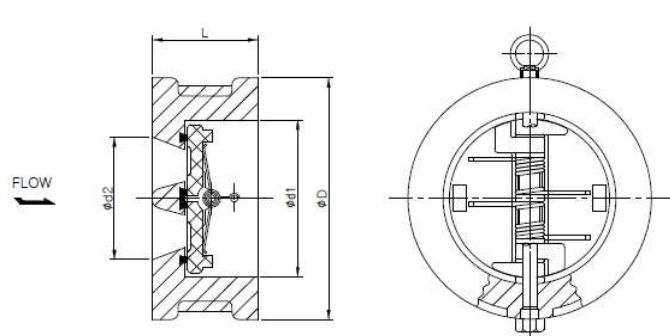
WAFER
